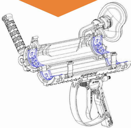
BAABS Long Rail Assembly w/ Electric G3 Trigger Deadman & Adjustable Brace
