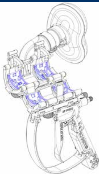
Compact BAABS Assembly w/ Pneumatic G3 Trigger Deadman
